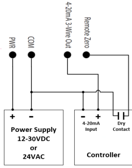
3 – Wire 4 – 20mA
