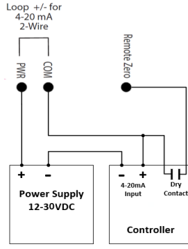
2 – Wire 4 – 20mA
